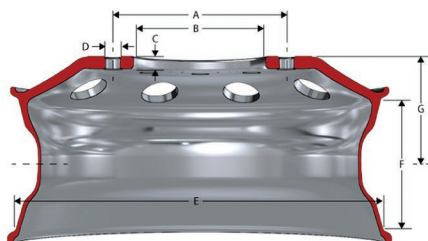
Typical Wheel Shown - Dimensional Reference Only
